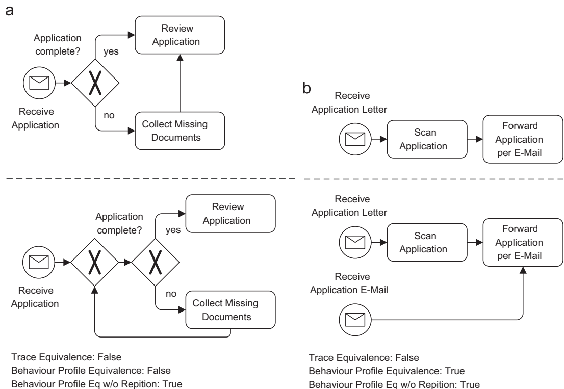
Fig. 4. Two objects of our experiment illustrating a difference related to an activity (event, respectively) that is (a) part of a correspondence, (b) not part of a correspondence.
