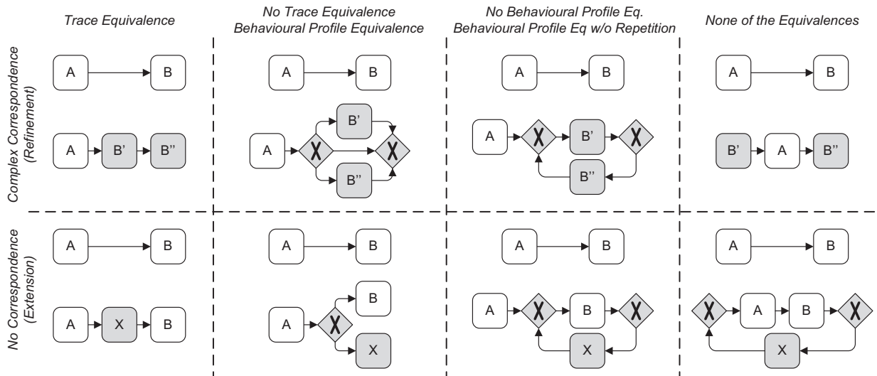
Fig. 3. Overview of correspondences with respect to their behaviour preserving properties.
