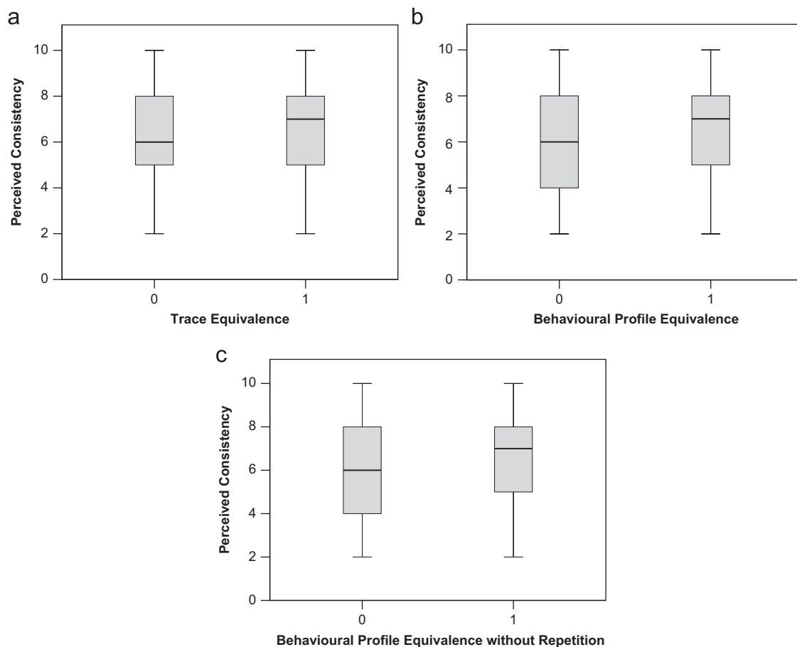
Fig. 6. Trace Equivalence (a), Behavioural Profile Equivalence (b), and Behavioural Profile Equivalence without Repetition (c) versus Perceived Consistency.
